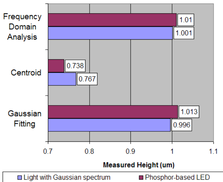
Fig. 11. Comparing measurement accuracy of different algorithms between different light sources, ideal value is 1um.
