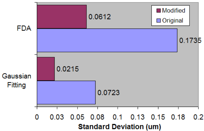
Fig. 15. Simulation verification on the proposed modification: Comparing standard deviation of measuring perfectly flat surface reproduced by proposed modification and original.
