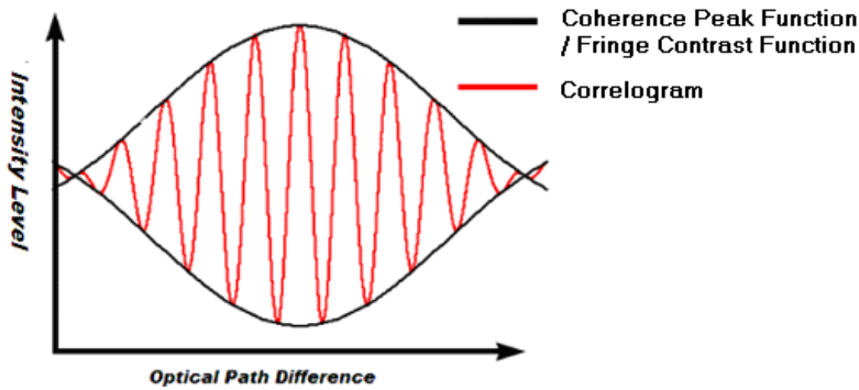
Fig. 3. Example of correlogram and corresponding fringe contrast function (also known as coherence peak function) in vertical scanning interferometry.
