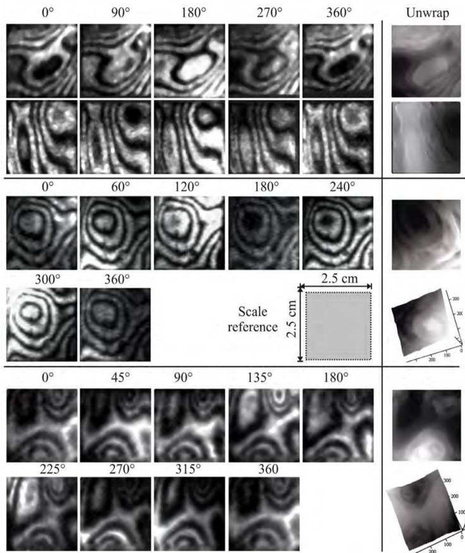
Fig. 9. Flow of oil drops on glass. Phase-shifted interferograms and unwrapped phases. Upper two rows: two examples of five 90^\circ phase-shifts. Center rows: seven 60^\circ phase-shifts. Lower rows: nine 45^\circ phase-shifts. Reference square for scale dimensions.
