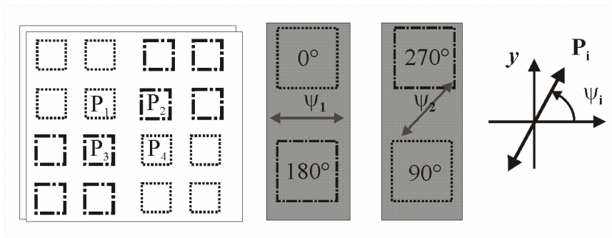
Fig. 5. Polarizing filters array for 90° phase stepping.
