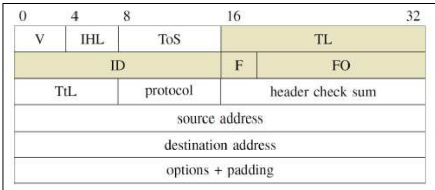
Fig. 9. IP header. Shaded fields are used in the defragmentation process. Legend: V: protocol version; IHL: Internet Header Length; ToS: Type of Service; TL: Total Length; ID: Identification Data; F: Flags; FO: Fragment Offset; TTL: Time to Live.
