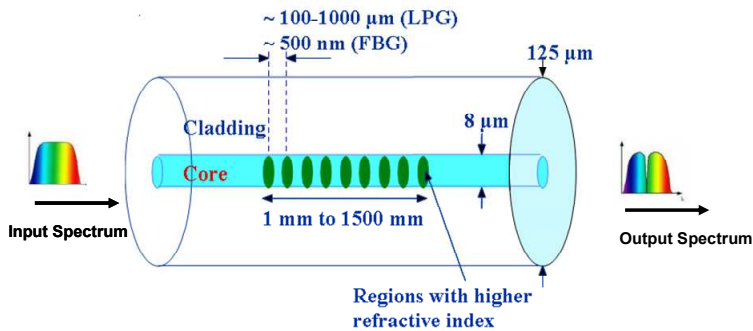
Fig. 1. Schematic representation of a fiber grating
