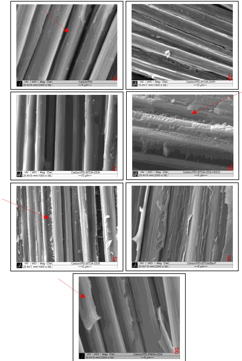
Fig. 8. The fracture surface of the manufactured composites with: a) the hot compression molding and aqueous suspension prepregging b) PI-BTDA/DHP; c) PI-BTDA/ODA; d) PI-BTDA/ODA-treated fiber with HNO 3 ; e) PI-BTDA/DDS; f) PI-BTDA/BisP and, g) PI-PMDA/ODA.
