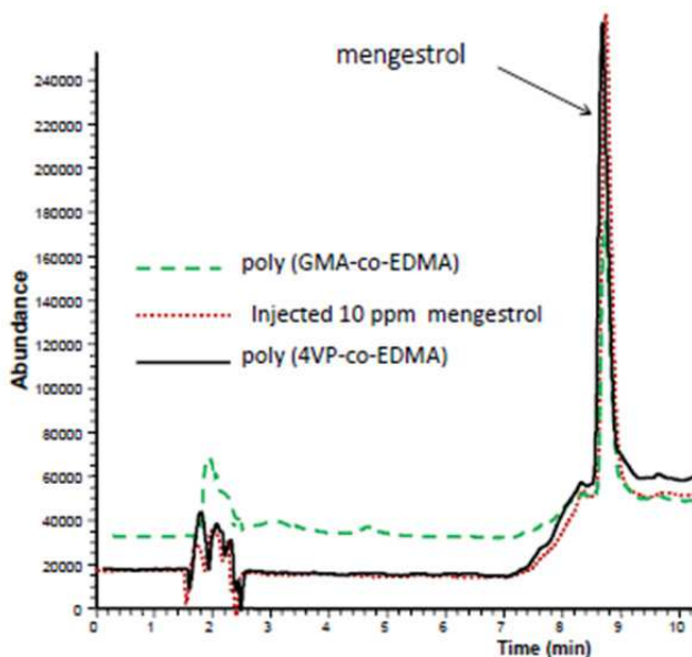
Fig. 8. Overlapped chromatogram indicating meggestrol peak for poly( 4VP-co-EDMA) and poly (GMA-co-EDMA) and directly injected 10 ppm meggestrol standard.
