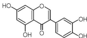
Fig. 2. Structure of orobol (5,7,3',4'-tetrahydroxyisoflavon).
