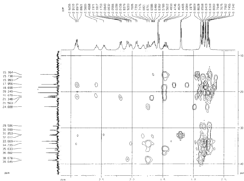
Fig. 10. Lygosteroside B (HMBC).
