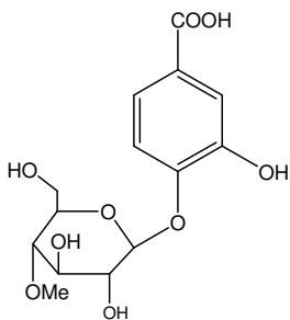
3,4-Dihydroxybenzoic acid 4-O-(4'-O-methyl)- \beta -D-glucopyranoside
