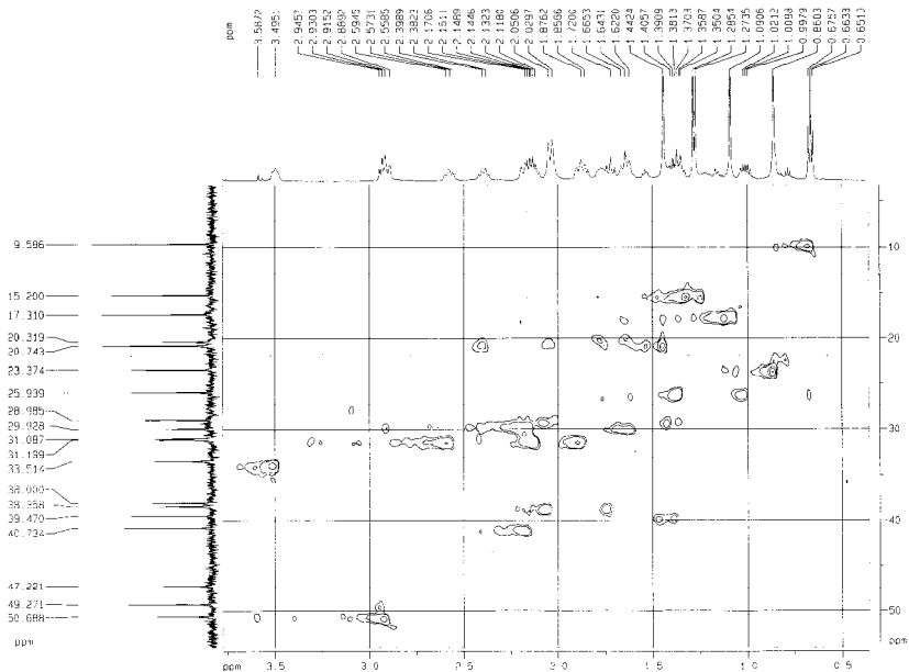
Fig. 21. Lygosteroside A (HSQC, in C_5D_5N ).
