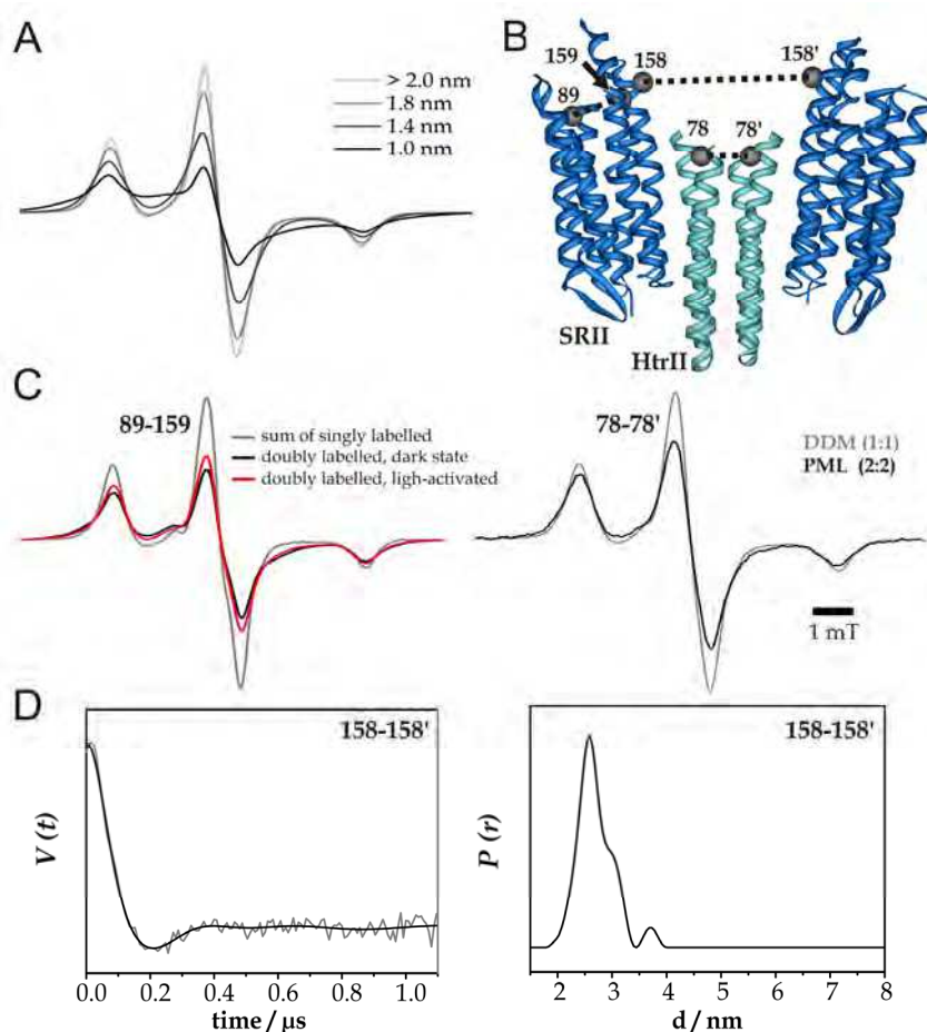
Fig. 6. Interspin distance measurements. (A) Simulated powder spectra (obtained by cw EPR on frozen samples) for different interspin distances. (B) Ribbon representation of the X-ray structure of the 2:2 NpSRII-NpHtrII complex (PDB 1H2S). Positions L89, S158 and L159 in NpSRII , and V78 in NpHtrII are shown as spheres. (C) left: cw EPR spectra ( T = 160 K) of the double mutant L89R1/L159R1 in the receptor ground state (black) and in the trapped signaling state (M-state, red) compared to the sum of the spectra of the singly labeled samples (gray) reveals line broadening due to dipolar interaction. Interspin distances of 1.1 ( \pm 0.2 ) nm for the ground state and 1.3 ( \pm 0.2 ) nm for the M-trapped have been determined (Bordignon et al., 2007); right: NpHtrII-V78R1 solubilized in DDM (gray) or reconstituted in PML (black) in the absence of NpSRII . The interspin distance obtained in the reconstituted sample is 1.3 ( \pm 0.2 ) nm (Klare et al., 2006). (D) Left: background corrected DEER time domain for NpSRII-S158R1 . The distance distribution shown in the right panel shows a mean distance of 2.6 nm between the two spin labels bound to positions 158 in the 2:2 complex that is in good agreement with the distance of 3 nm between the oxygen atoms of the respective serine residues as calculated from the crystal structure.
