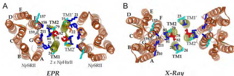
Fig. 7. (A) EPR based model of the transmembrane region of the NpSRII / NpHtrII complex (viewed from the cytoplasmic side). Side chains where spin labels have been attached are shown in stick representation. The color code represents the strength of the observed dipolar interaction (blue and red: strong; cyan and orange: weak). (B) Crystal structure of NpSRII / NpHtrII (PDB: 1H2S) (Klare et al., 2004). The color code for the side chains is the same as in (A).
