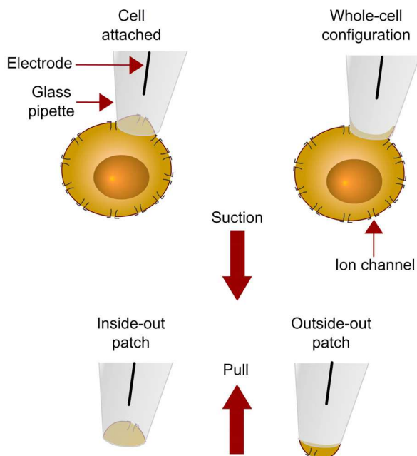
Fig. 2. Illustration of the different modes and configurations of the patch-clamp technique. In the cell-attached mode, the patch electrode remains sealed to the cell membrane, permitting the recording of currents through single-ion channels from the patch of membrane surrounded by the tip of the electrode. This configuration can be used for studying the activity of ion channels present in the membrane patch. In the whole cell mode, in the initial cell-attached configuration, additional suction is applied to rupture the cell membrane, thus providing access to the intracellular space. The larger opening at the tip of the patch electrode, compared with the sharp microelectrode, provides lower resistance and better electrical access to the cell- because the volume of the patch electrode is much bigger than the cell, cellular soluble contents will slowly be replaced by contents of the electrode, referred to as “dialyzing” the cell contents. Whole-cell mode records currents through all channels from the entire cell membrane at once. In the Inside-out patch mode, after the gigaseal are formed, the micropipette is quickly withdrawn from the cell, pulling off a patch of membrane from the cell, leaving the membrane patch attached to the micropipette, and exposing the intracellular surface of the membrane to the external media. This is useful when an experimenter wishes to pharmacologically manipulate the intracellular side of the ion channels. In the outside-out mode, after the whole-cell patch is formed, the electrode can be slowly withdrawn from the cell, allowing a bulb of membrane to bleb out from the cell. After the electrode to be pulled far enough away, this bleb will detach from the cell and reform as a convex membrane at the electrode end (like a ball open at the electrode tip), with the original outside of the membrane facing outward from the electrode. Single channel recordings are possible in this form if the membrane bleb is small enough. Outside-out patching gives the experimenter the opportunity to examine the properties of an ion channel when it is isolated from the cell, and exposed to different solutions on the extracellular membrane surface.
