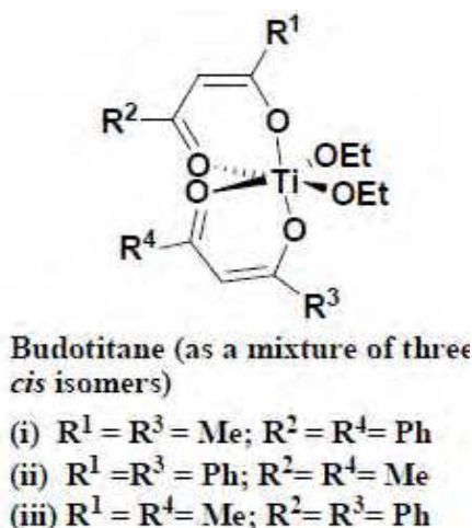
Fig. 11. The molecular structure of budotitane (Bharti & Singh, 2009).
