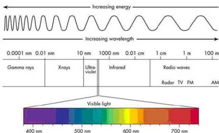
Fig. 1. Electromagnetic wavelength
