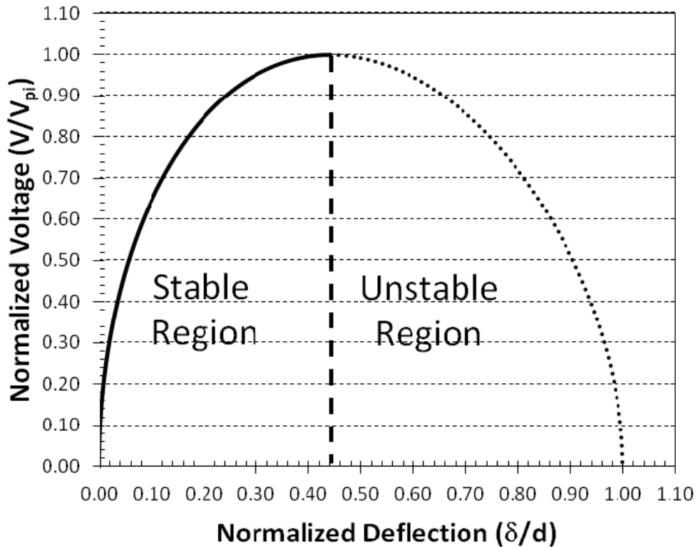
Fig. 5. Stable and Unstable Regions of Bisection Model.
