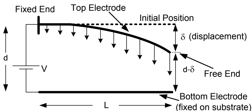
Fig. 1. Electrostatic actuator (Side View)
