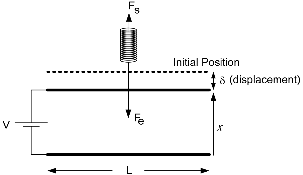
Fig. 2. Lumped model of a cantilever actuator.
