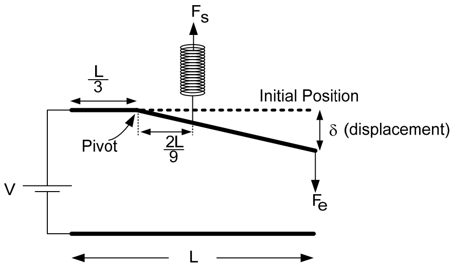
Fig. 3. New Approach (Bisection Model) to cantilever actuator.
