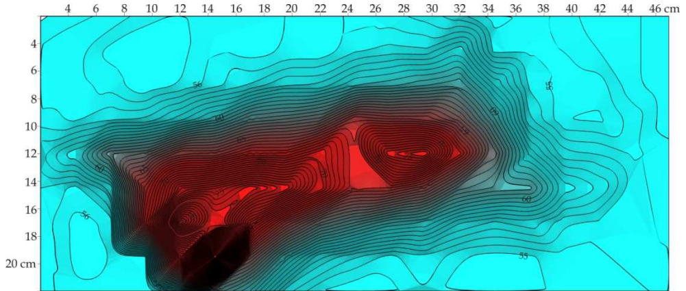
Fig. 7. Contour plotting of transmission times ( \mu s) taken from top of the model
