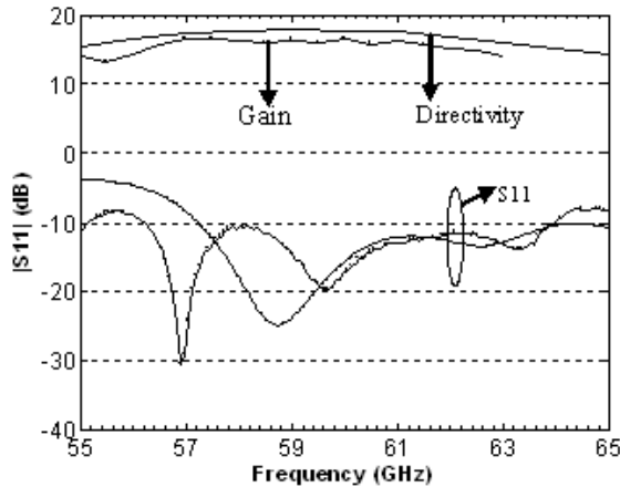
Fig. 27. Variation of S11 and gain for a 2 x 2 superstrate aperture antenna array. Simulation —; measurement - - - .
