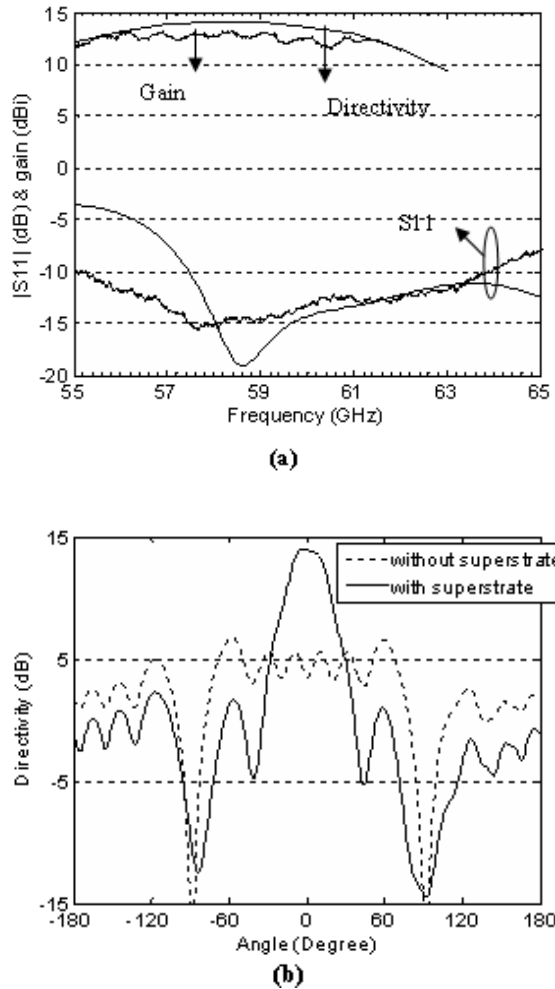
Fig. 23. (a) Results of S11 and gain with a superstrate dimension of 1.2 \lambda_0 \times 2.7 \lambda_0 . Simulation —•—; measurement —. (b) Simulated comparison of E-plane antenna radiation pattern with and without superstrate.
