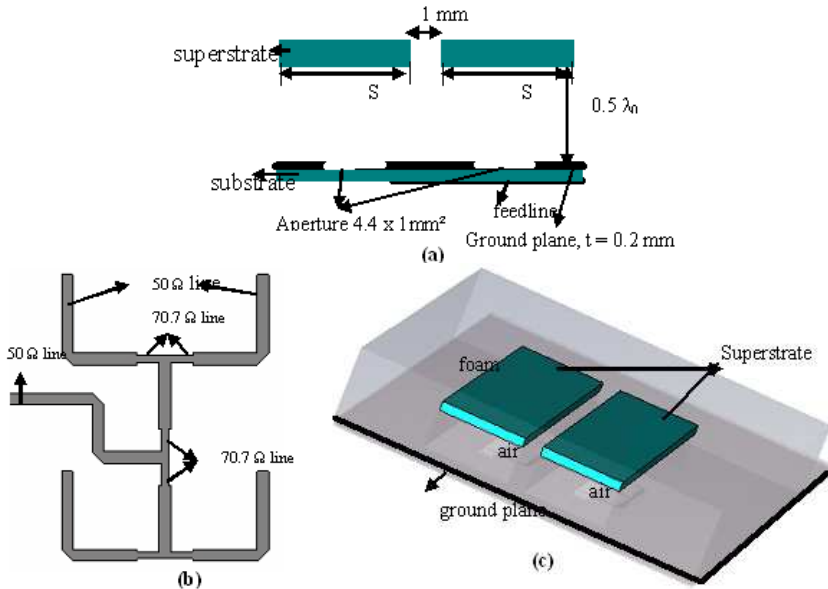
Fig. 25. (a) Cutting plane of a 2 \times 2 aperture antenna array with superstrate, ground plane size = 6 \lambda_0 \times 10 \lambda_0 for connecting V band connector and for ease of measurement purpose. (b) 2 \times 2 feed network. (c) Overview of 2 \times 2 array prototype: details of the two separate superstrate sheets and air gap within foam.
