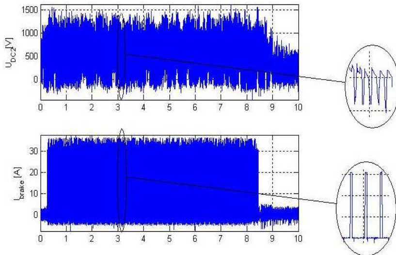
Fig. 5. Example of the measured DC current and DC voltage with the Yokogawa PZ4000 power analyzer during a lowering motion (Minav, 2011d).
