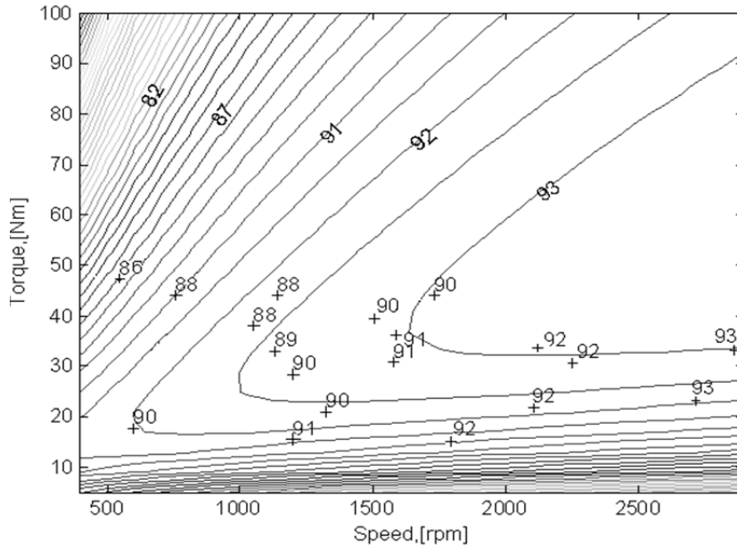
Fig. 6. Efficiency of the 10 kW CFM112M PMSM (solid line). Some measured efficiency points in lifting are indicated by + signs (Minav, 2011a).
