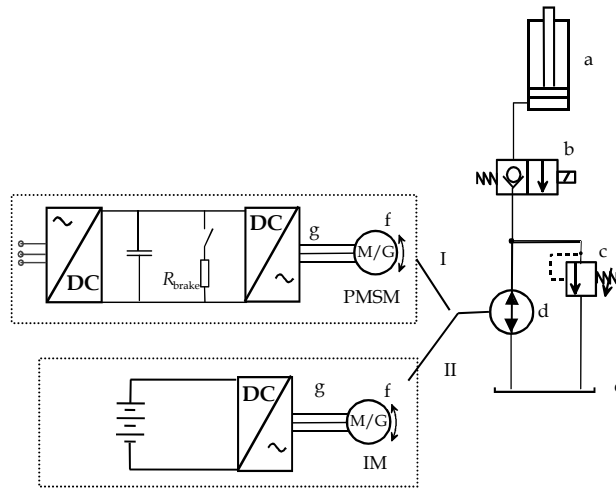
Fig. 2. Structures of the hydraulic and electric system to be tested. The experimental system consists of: a) single-acting cylinder, b) two-way normally closed poppet valve, c) pressure relief valve, d) hydraulic machine acting both as a pump or a motor, e) oil tank, f) electric machine operating both as a motor or a generator, g) frequency converter, and brake resistor R_{\text{brake}} (Minav, 2008).
