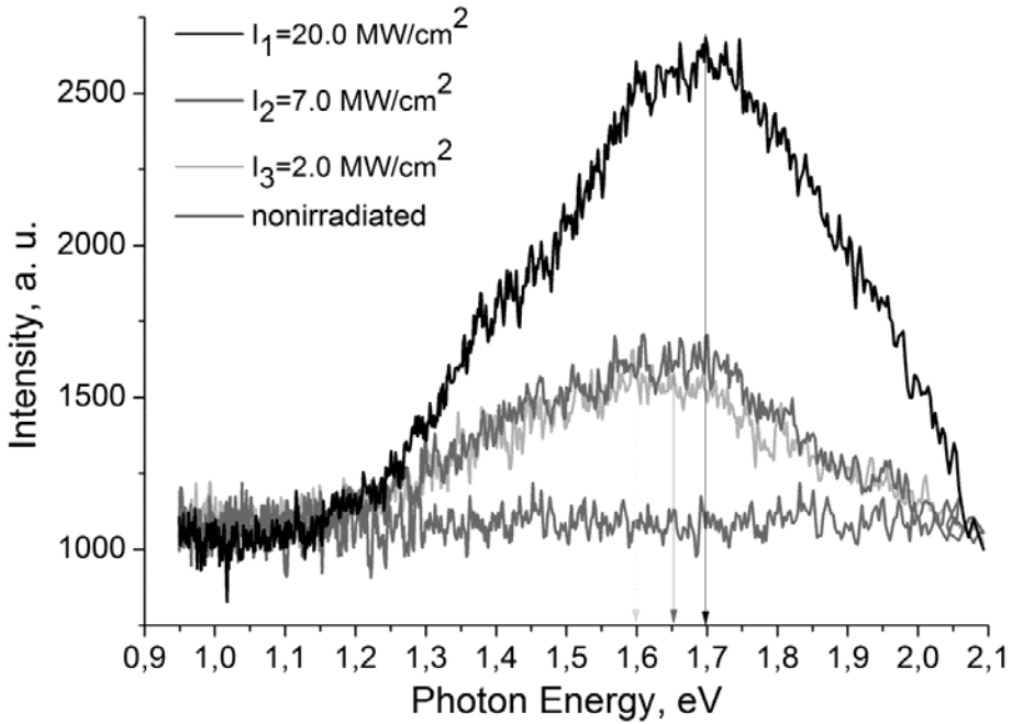
Fig. 19. Photoluminescence spectra of Si_{0.7}Ge_{0.3}/Si heteroepitaxial structures before and after irradiation by Nd:YAG laser.
