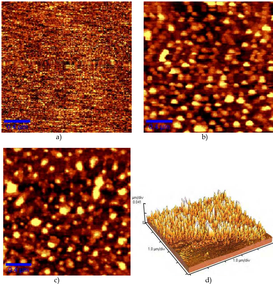
Fig. 11. Atomic force microscope images of ITO/p-Si structure: a) non-irradiated, irradiated by Nd:YAG laser at intensities of b) 1.13 MW/cm 2 ; c) 2.83 MW/cm 2 and d) boarder of non-irradiated (smooth surface) and irradiated by Nd:YAG laser at intensity 2.83 MW/cm 2 (surface with nanocones).
