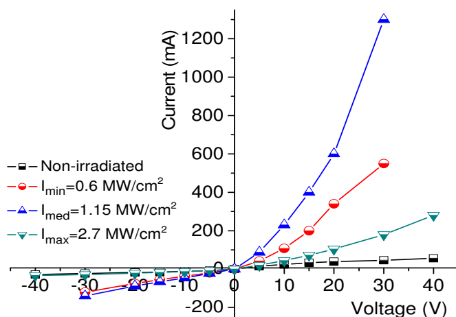
Fig. 1. Current-voltage characteristics of a non-irradiated and irradiated i-Ge sample by Nd:YAG laser with different intensities of quantum energy h\nu_4=4.66 eV and 350 laser pulses.
