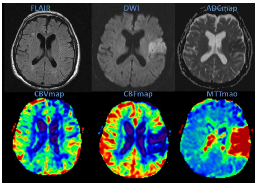
Fig. 4. Imaging of an acute ischemic lesion in a 45 yrs old female with NPSLE and antiphospholipid syndrome (APS), 4 hours after the onset of the symptoms. FLAIR is unremarkable, while the lesion is revealed on DWI and ADC map as hyperintense and hypointense area, respectively, due to cytotoxic edema. Dynamic Susceptibility Contrast (DSC) MR Perfusion technique shows mild increased cerebral blood volume (red on CBV map), decreased cerebral blood flow (dark blue on CBF map) and increased mean transit time (red on MTT map)
