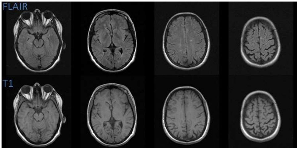
Fig. 1. FLAIR and T1 MR images of a 44 years female with NPSLE reveal multiple focal punctate lesions-hyperintense on FLAIR and hypointense or isointense on T1- at the periventricular and subcortical white matter, semioval center and the cortex of the left frontal lobe.
