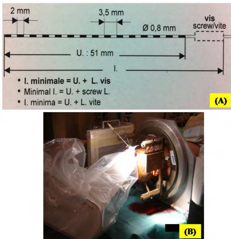
Fig. 3. (A) Drawing of an electrode with 15 contacts: U.: electrode length of 15 contacts = 51 mm, \varnothing : diameter of the electrode = 0.8 mm, length of each contact = 2 mm, distance between the two contacts = 1.5 mm. (B) Robotic arm: in the position of an anterior (trans opercular) oblique insular electrode trajectory.
