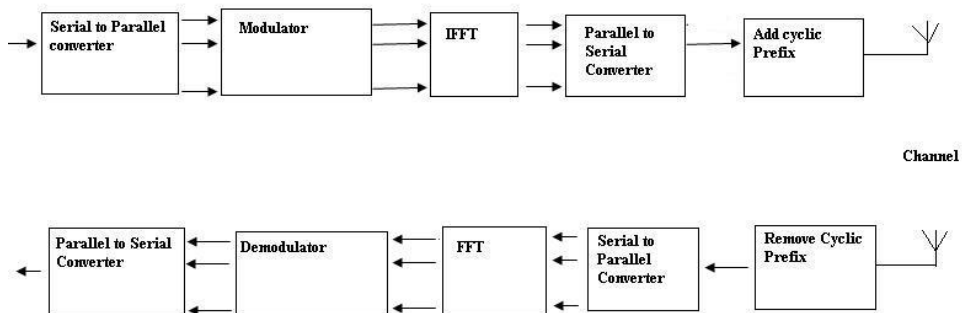
Fig. 1. OFDM system
