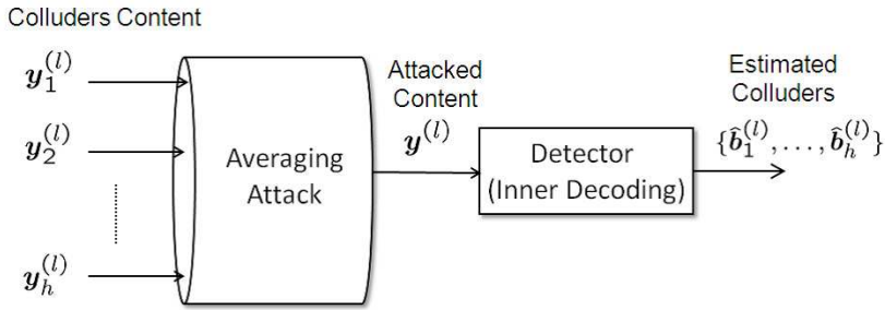
Fig. 2. Illustration of the averaging attack at segment l conducted by \mathcal{S}_c = \{1, 2, \dots, h\} . The sequence \hat{b}_j^{(l)} is an estimate which corresponds to b_j^{(l)} .
