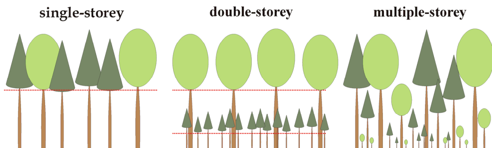
Fig. 4. Quantification of vertical diversity.
