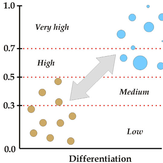
Fig. 3. Schematic visualisation of the assessment of stand differentiation according to Fuldner (1995) with categories proposed by Aguirre et al. (1998).
