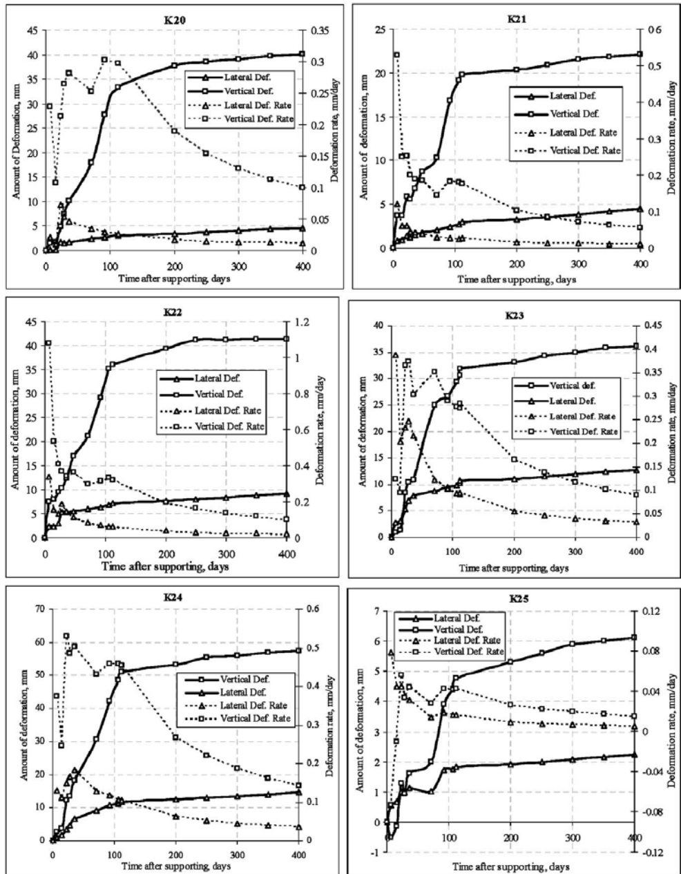
Fig. 10. Convergence versus time at the hanging wall stations (Onargan et al, 2004).
