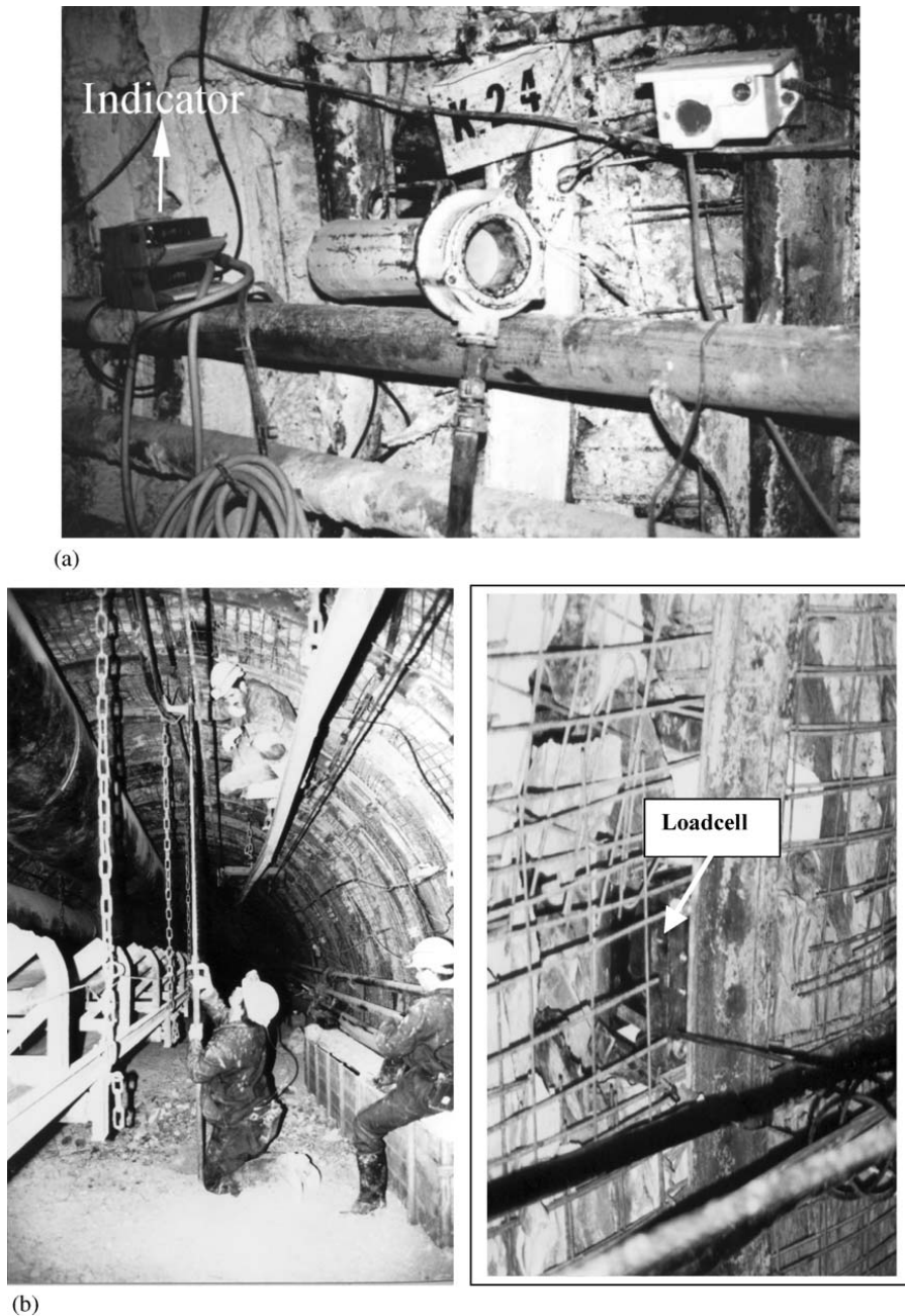
Fig. 8. Some views of the measurement stations in the hanging-walls: (a) a view of the station (K-24) and (b) convergence and support load measurement studies (Onargan et al., 2004).
