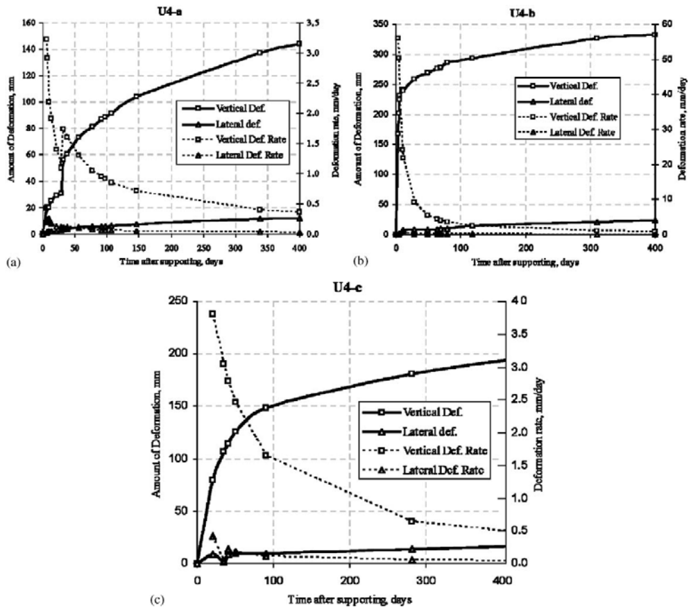
Fig. 9. Convergence versus time at the soda beds: (a) U4-a station (Steel set spacing 0.5 m), (b) U4-b station (Steel set spacing 1.00 m) and (c) U4-c station (steel set spacing 0.70 m). (Onrgan et all, 2004).
