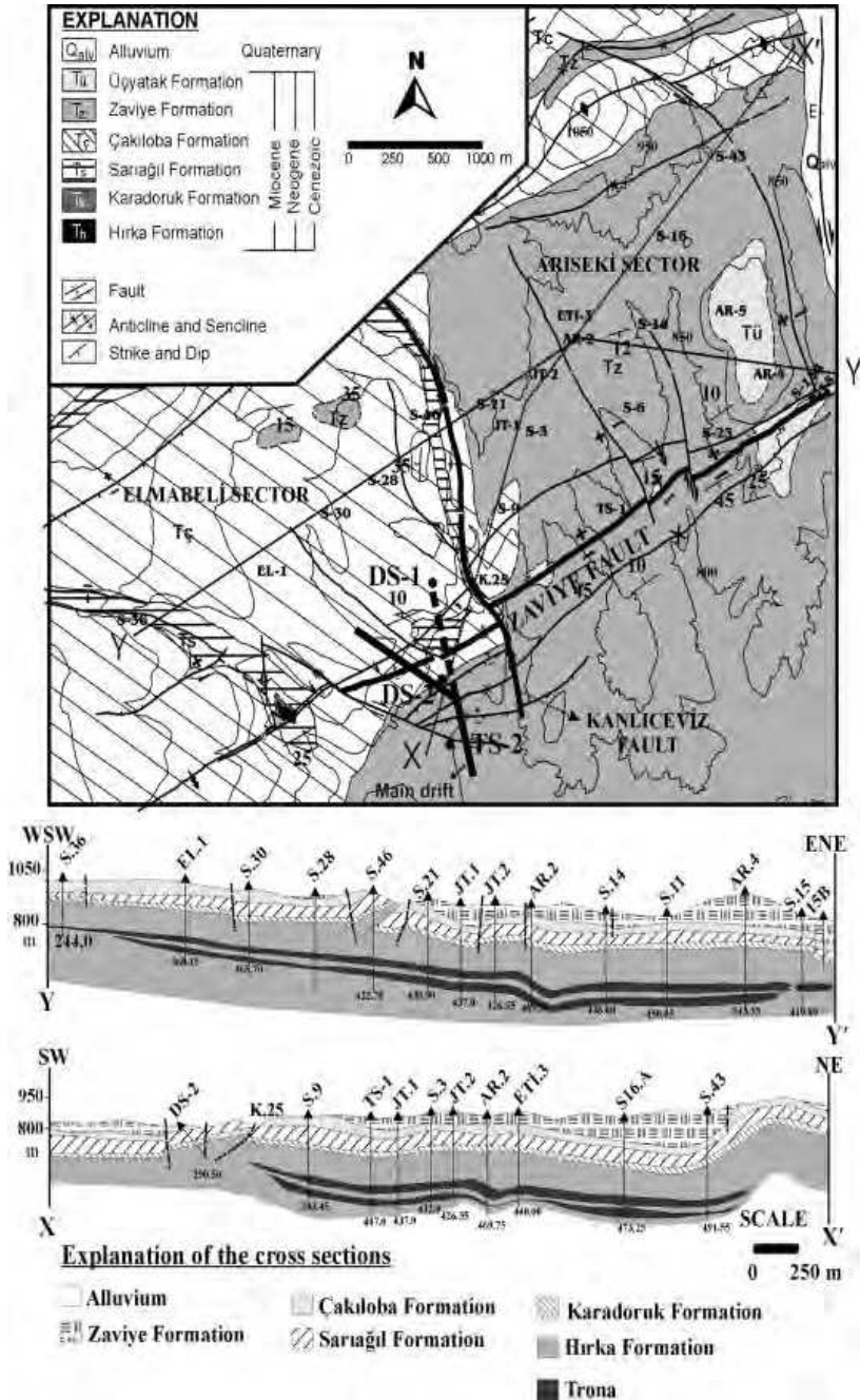
Fig. 2. Geological map and cross-sections of the Bey pazari natural soda field (Onargan et al, 2004).
