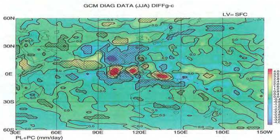
Fig. 3. The same as in Fig. 2, except for the differences between GR and CN.
