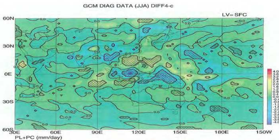
Fig. 2. Comparison of the JJA mean values of precipitation of the impact experiments with those of the control integration (impact - control). The differences between C4 and CN are indicated. The results for the experiment areas and the surrounding areas are indicated. The colors toward red indicate relatively large values. The areas where the Student's t -test values indicate statistically significant differences (at the 95 % level) are hatched.
