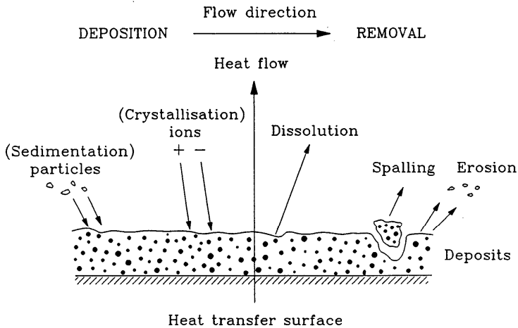
Fig. 2.1. Various deposition and removal processes during fouling.
