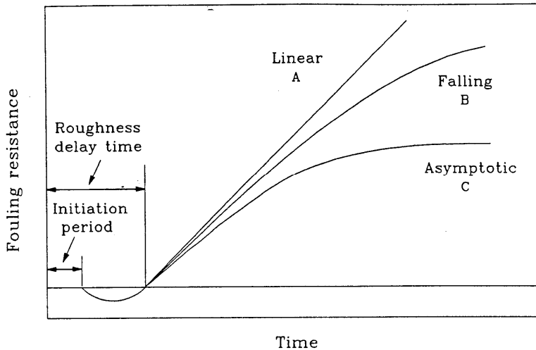
Fig. 2.2. Typical fouling curves.
