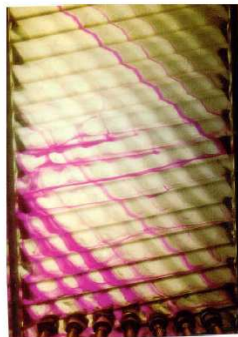
Fig. 11B. Flow visualization by Focke & Knibbe[7], Re=125 .
