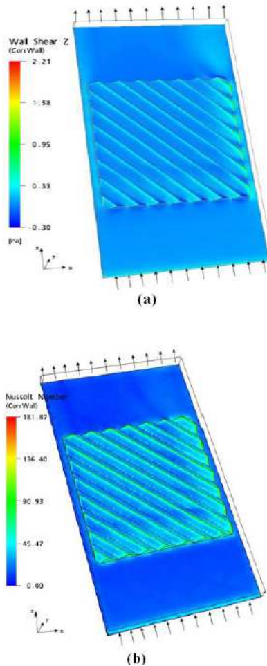
Fig. 13. Typical results of the CFD simulation for Re=900 ; distributions of: (a) z-shear stress component, (b) local Nusselt number.
