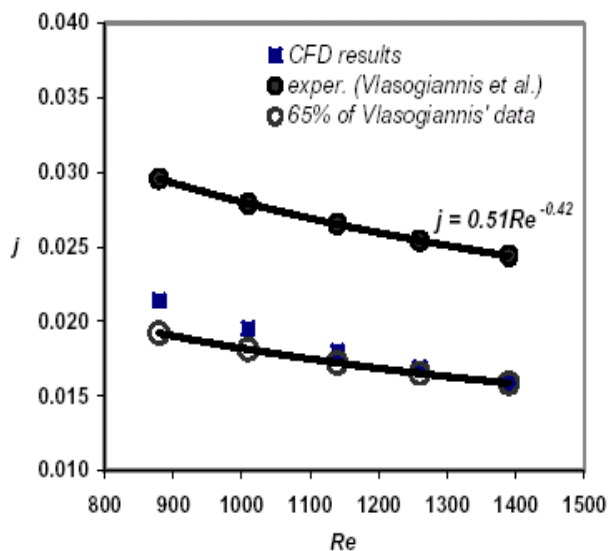
Fig. 15. Comparison of j -Colburn factor predictions (CFD) with experimental data.
