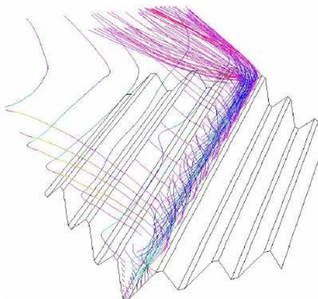
Fig. 12. Swirling flow inside a furrow; Re=900 .
