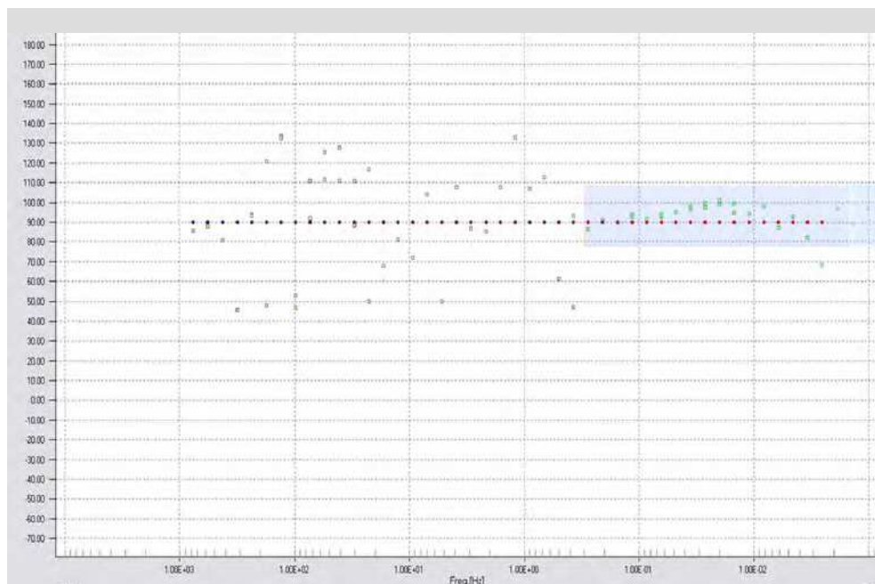
Fig. 6. Strike orientation (degrees) versus frequency (Hz): blue rectangle delineates the frequency range for 2D structure with average strike orientation of \text{N}96^{\circ}\text{E}
