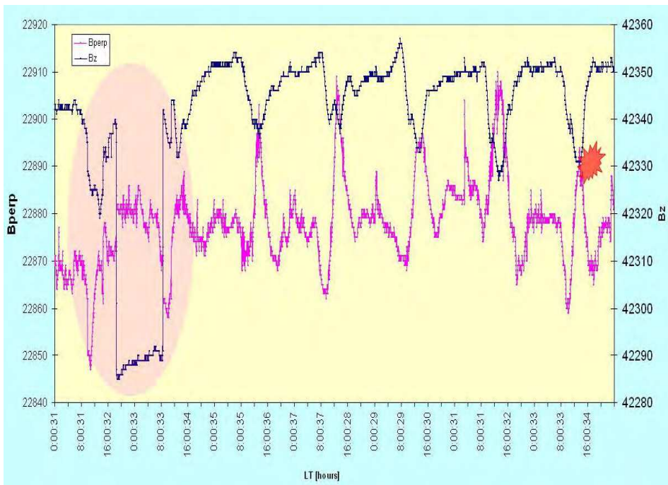
Fig. 8. Geomagnetic time series (Bperp and Bz) recorded at the GOPS for 7 days interval (April19- April 25, 2009); Bperp is B_{\perp} ; red star is earthquake of M5.0; pink ellipse marks a pre-seismic disturbance of the vertical component (Bz) of geomagnetic field (lead time is about 6 days before the earthquake).
