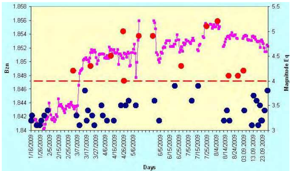
Fig. 14. Distributions of the normalized function Bzn and earthquake magnitude on the 2009 analyzed interval; blue circles are earthquakes with M < 4 ; red circles are earthquakes with M \geq 4 ; red dashed line represents the limit above to which one earthquake of M \geq 4 is possible to occur.
