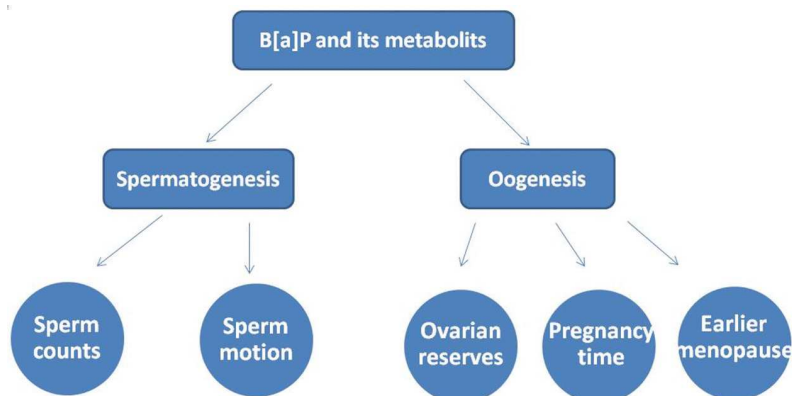
Fig. 2. Influence of benzo[a]pyrene on male and female fertility.
