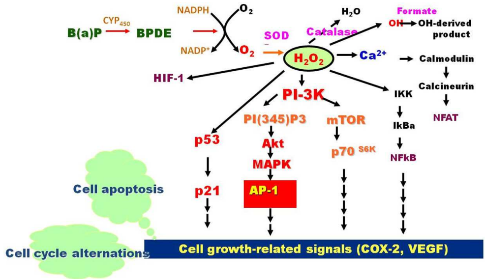
Fig. 3. Mechanism of benzo(a)pyrene-related reproduction toxicity.
