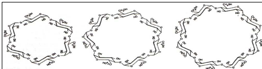
Fig. 1. Chemical structures of (a) \alpha CD; (b) \beta CD; (c) \gamma CD
