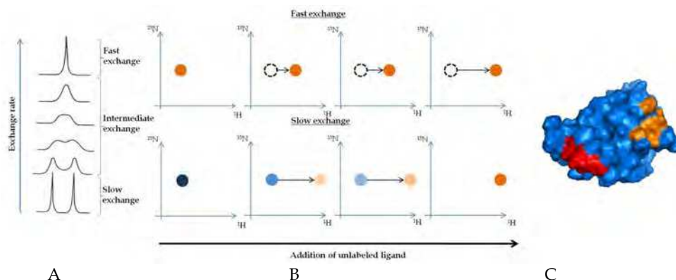
Fig. 3. Mapping of binding sites by NMR. (A) In the presence of free and ligand-bound proteins, the NMR signal varies as a function of the exchange rate. Its chemical shifts and linewidths evolve from a FAST exchange to a SLOW exchange condition. When the exchange is FAST, only one averaged chemical shift is observed. When it is SLOW, the chemical shifts corresponding to the free and bound forms are observed. (B) The chemical shift changes measured during the titration of a labelled protein with its binding partner are displayed in the case of FAST exchange (upper panel) and SLOW exchange (lower panel). (C) Residues whose NMR chemical shifts and/or linewidths change during the titration with ligands A and B are colored in red and orange, respectively, on the surface representation of the 3D structure of the labelled protein. This “chemical shift mapping” study shows that the labelled protein recognizes its two ligands by different surfaces.
