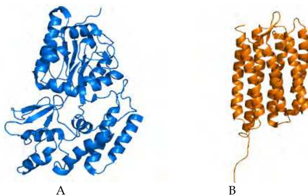
Fig. 1. Ribbon representation of the solution NMR structures of (A) the maltodextrin-binding protein (PDB ID 2KLF; Madl et al., 2009) and (B) the phototaxis receptor rhodopsin II (pSRII) from Natronomonas pharaonis (PDB ID 2KSY; Gautier et al., 2010).
