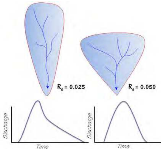
Fig. 9. Representation for two basins with different elongation ratio.
