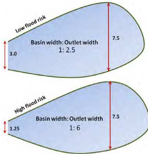
Fig. 8. Representative figure showing the widths of upstream and out let.
