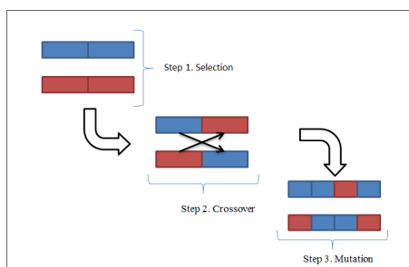
Fig. 4. Basics steps of a Genetic Algorithm
