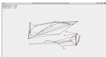
Fig. 17. Generation 500, graph 17470
