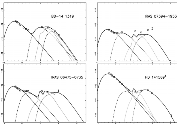
Fig. 4. GA SEDs obtained the stars BD-14 1319, IRAS 07394-1953, IRAS 06475-0735 and HD 141569. The plots are given as \log[\lambda F_\lambda(Wm^{-2})] versus \log[\lambda(\mu m)] (Hetem & Gregorio-Hetem 2007).
