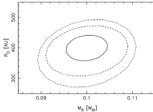
Fig. 3. Contour levels gof(M_D, R_D) estimated for AB Aurigae presenting the confidence levels \chi^2(68\%)=0.082 (continuous line), \chi^2(90\%)=0.15 (dashed) and \chi^2(99\%)=0.21 (Hetem & Gregorio-Hetem 2007).
