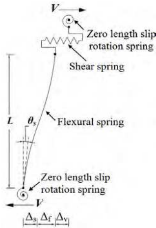
Fig. 6. Spring representation of total response model
