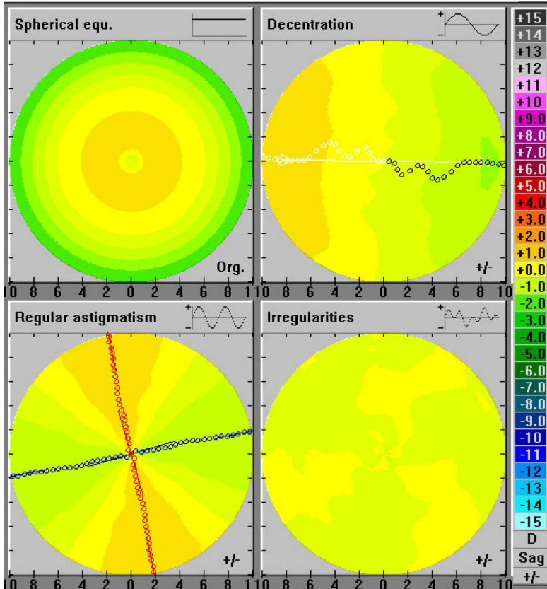
Fig. 6. Fourier analysis of a normal corneal topography
