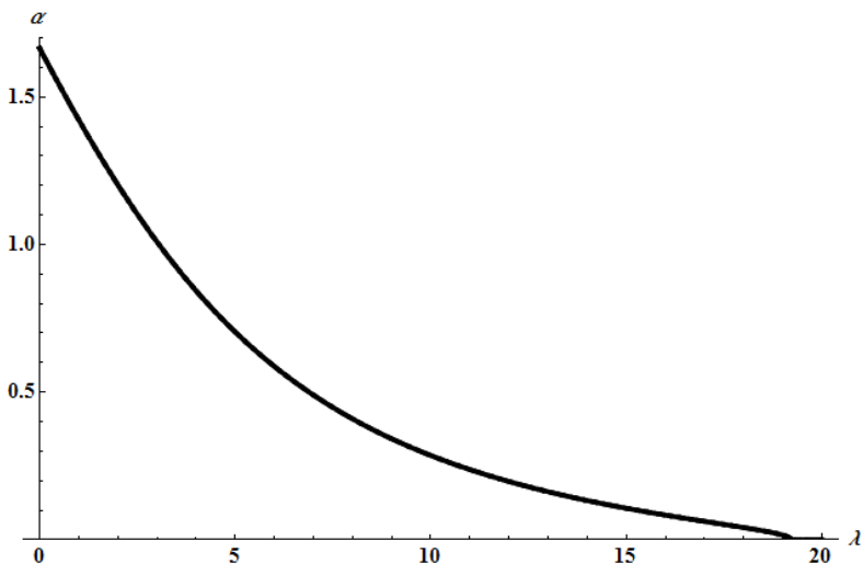
Fig. 3. \alpha = d\theta(0)/dx against \lambda for the first fourth modes. These modes coincide for each of the values of \lambda .
