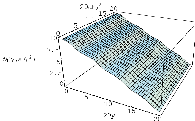
Fig. 4. Phase function \theta_1(y, aE_0^2) according to equation (41) inside the slab. Parameters as in figure 3.
