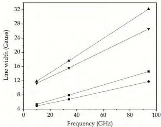
Fig. 8. Line width \Delta H of the free radical signal versus microwave frequency of EPR spectra recorded in the X-, Q- and W- bands at room temperature. \blacksquare , \Delta H_{pp} (Arabian petroleum); \bullet , \Delta H_{pp} (Colombian petroleum); \blacktriangle , \Delta H_{1/2} (Arabian petroleum); \blacktriangledown , \Delta H_{1/2} (Colombian petroleum).
