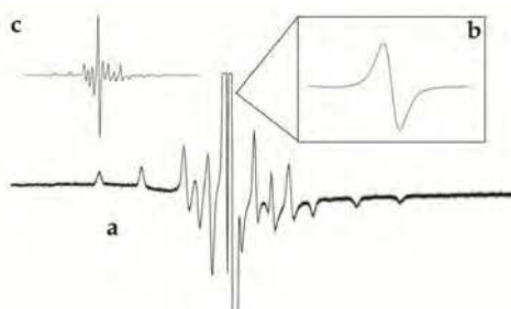
Fig. 5. a EPR spectrum for Brazilian crude oil; b Signal of the free radical; c Simulated spectrum for VO^{2+} (Guedes et al., 2001).
