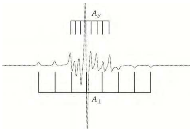
Fig. 10. Simulated spectra of \text{VO}^{2+} in crude oil and indication of lines corresponding to the parallel and perpendicular directions in relation to the applied magnetic field.
