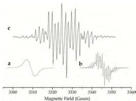
Fig. 22. Spectra subtraction for analysis of EPR hyperfine lines: a Unresolved line simulated by the software WINEPR SimFonia; b Overlap of the simulated spectrum and marine diesel spectrum at 383 K for subtraction of the unresolved line; c Result of the spectra subtraction.
