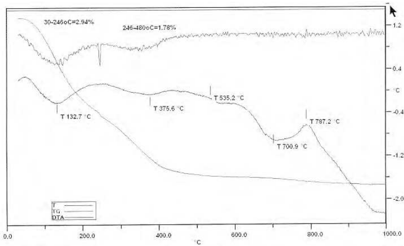
Fig. 7. DTA and DTG of glass FB2 system.
