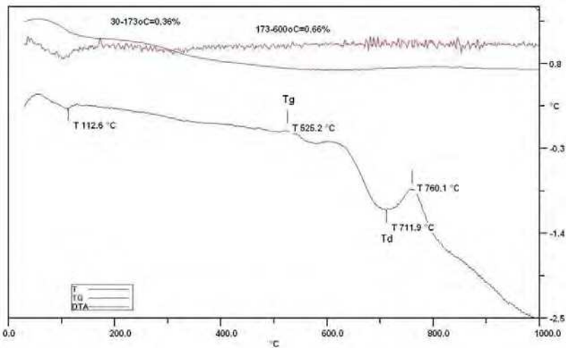
Fig. 8. DTA and DTG of glass FB3 system.
