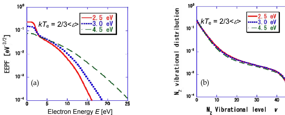
Fig. 15. (a) EEPF and (b) VDF of nitrogen plasma calculated numerically by the present scheme with pressure P = 1 Torr, T_g = 1200 K and N_e = 5.0 \times 10^{11} cm^{-3} .
