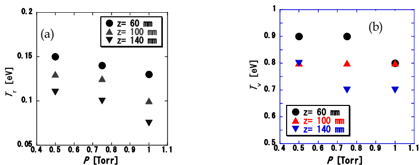
Fig. 4. (a) Rotational and (b) vibrational temperatures of C 3 Π u state of N 2 plasma measured experimentally, generated in the apparatus schematically shown in Fig. 3 ( \Delta v = -2 , v' = 0 , 1) (Sakamoto et al., 2007).
