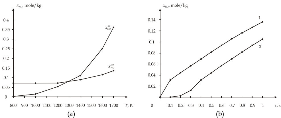
Fig. 2. Attainable equilibrium and extreme concentrations of NO as a function of temperature (a) and trajectory of attainment of x_{NO}^{ext} (b).
