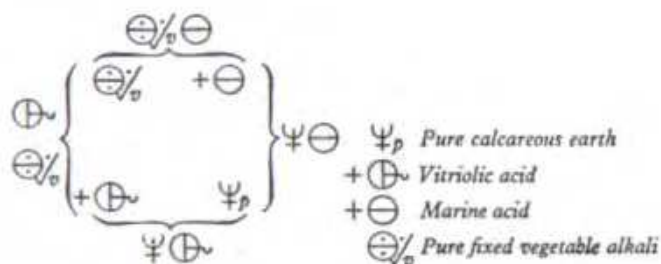
Fig. 2. This Affinity Diagram schematize two acid-base reactions
