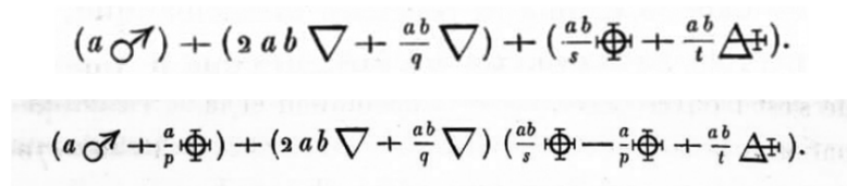
Fig. 3. Stoichimetric Equations with Lavoisier's symbols
