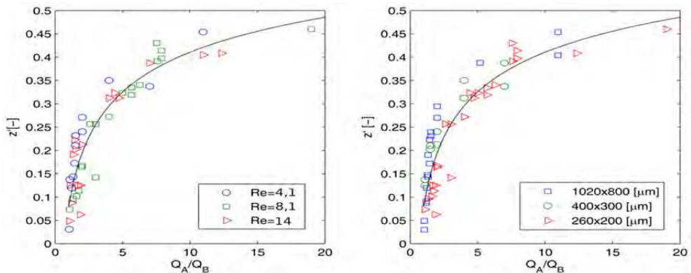
Fig. 14. Dimensionless pushing of the focused stream away from the channel axis as a function of the ratio of focused streams for different values of the Reynolds number (left-hand side diagram) and for channels of different dimensions (right-hand side diagram)
