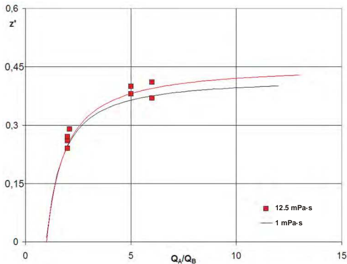
Fig. 17. The effect of liquid viscosity dimensionless pushing away of the focused stream from the channel axis for different values of the ratio of focusing streams
