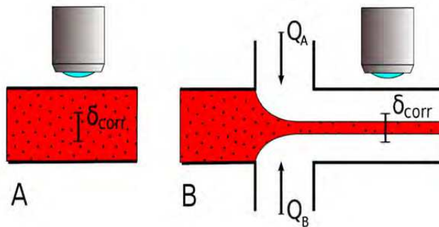
Fig. 19. The classical micro-PIV (A) and the idea of its modification as SeS-PIV (B)
