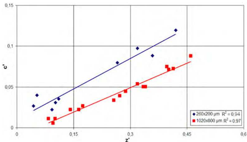
Fig. 15. Dimensionless deformation of focused stream c' as a function of dimensionless pushing off from the channel axis z' at constant Reynolds number Re=8.1
