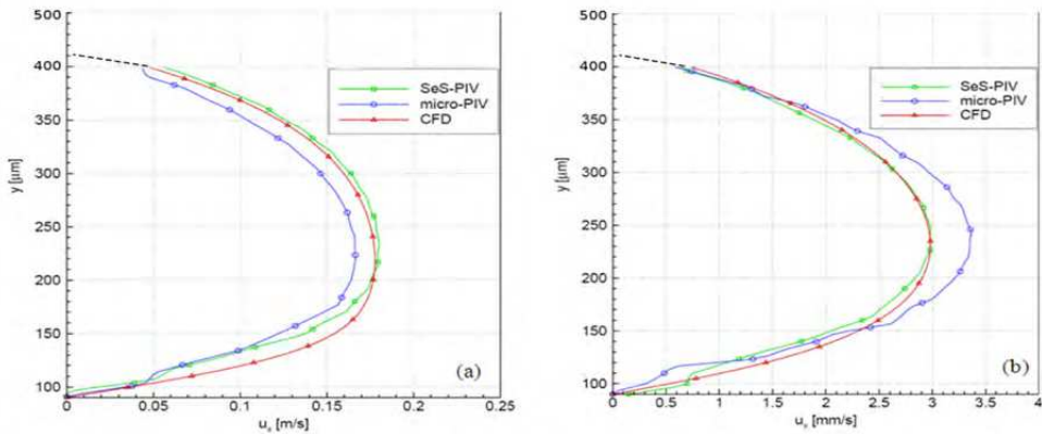
Fig. 22. Comparison of the numerical (CFD) and experimental results (SeS-PIV and micro-PIV) of vertical profile of velocity in the microchannel for Re=25 (left) and Re=0.4 (right)
