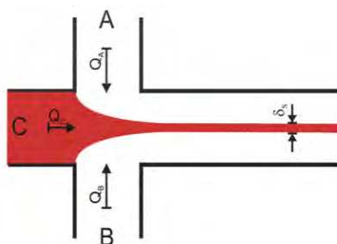
Fig. 1. Schematic view of hydrodynamic focusing in a four-channel intersection
