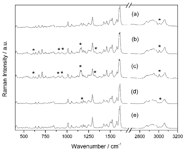
Fig. 8. Raman spectra of losartan potassium in association to hydrochlorothiazide in proportions: a) 1:1, b) 1:2, c) 1:4, d) 2:1 and 4:1.
