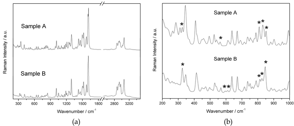
Fig. 4. Raman spectra of a) two crystalline phases (samples A and B) losartan potassium and b) a region of 200 to 1000 cm -1 .
