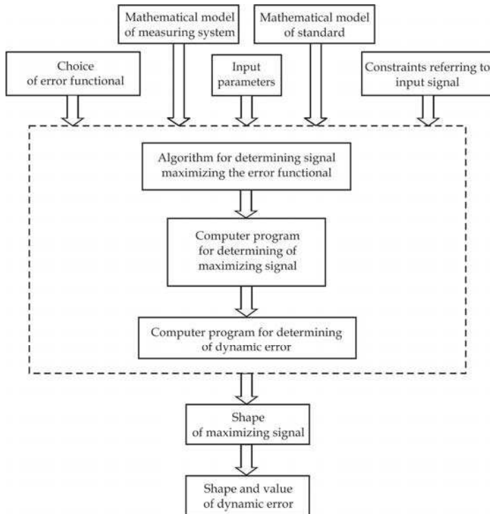
Fig. 1. Block diagram of calibration process of measuring systems based on maximum dynamic error.
