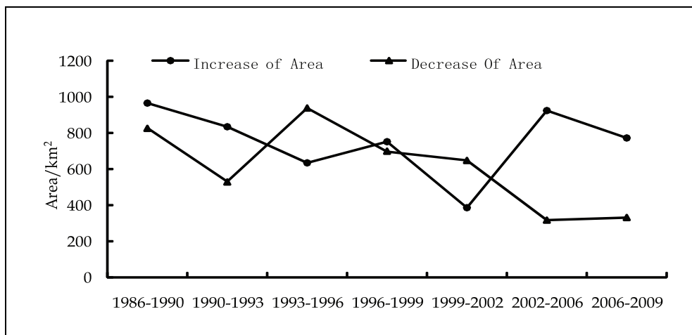
Fig. 7. The change of oasis area in each period in the Heihe River Basin (unit:km 2 )
