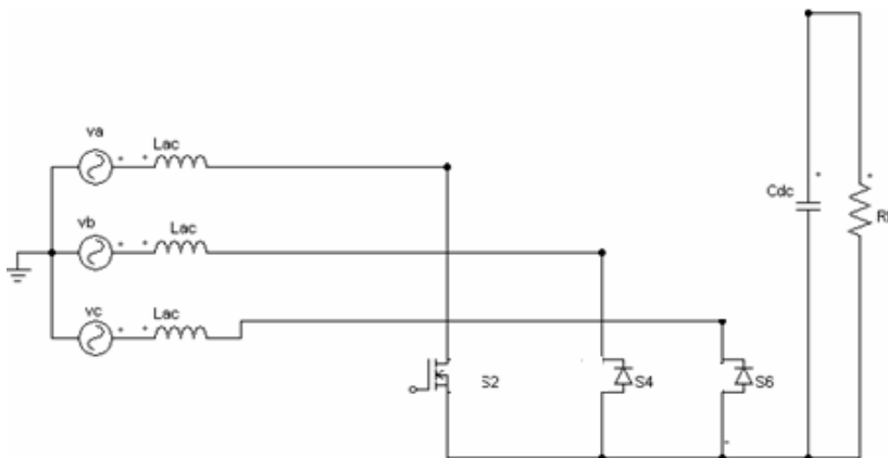
Fig. 2. Boost converter when V_a is positive.
