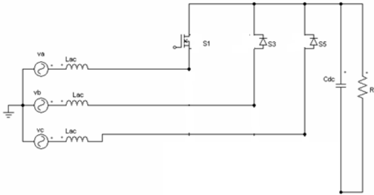
Fig. 3. Boost converter when V_a is negative.
