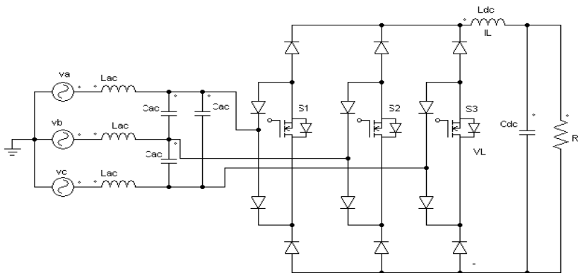
Fig. 4. Buck converter.
