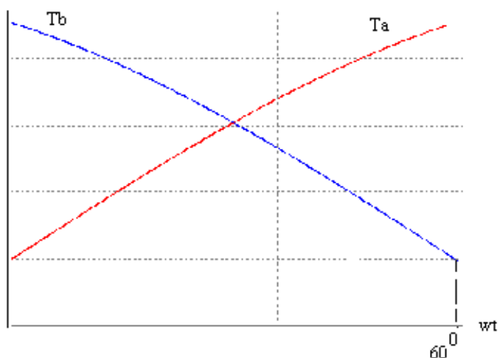
Fig. 5. Two 60° sine waves.
