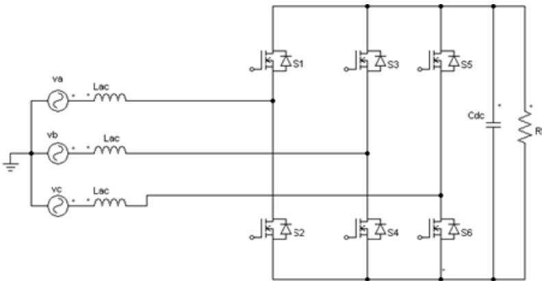
Fig. 1. Boost converter.
