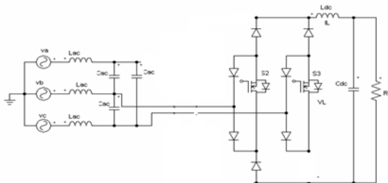
Fig. 7. Mode 2 equivalent circuit.
