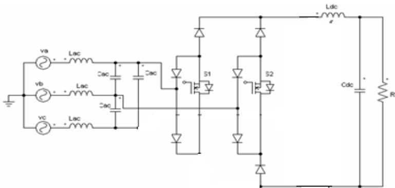
Fig. 6. Mode 1 equivalent circuit.
