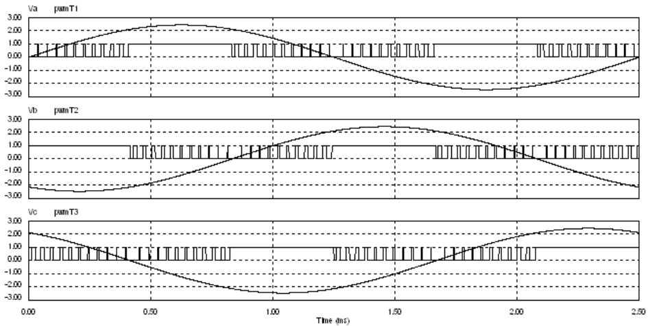
Fig. 9. PWM for the buck converter.
