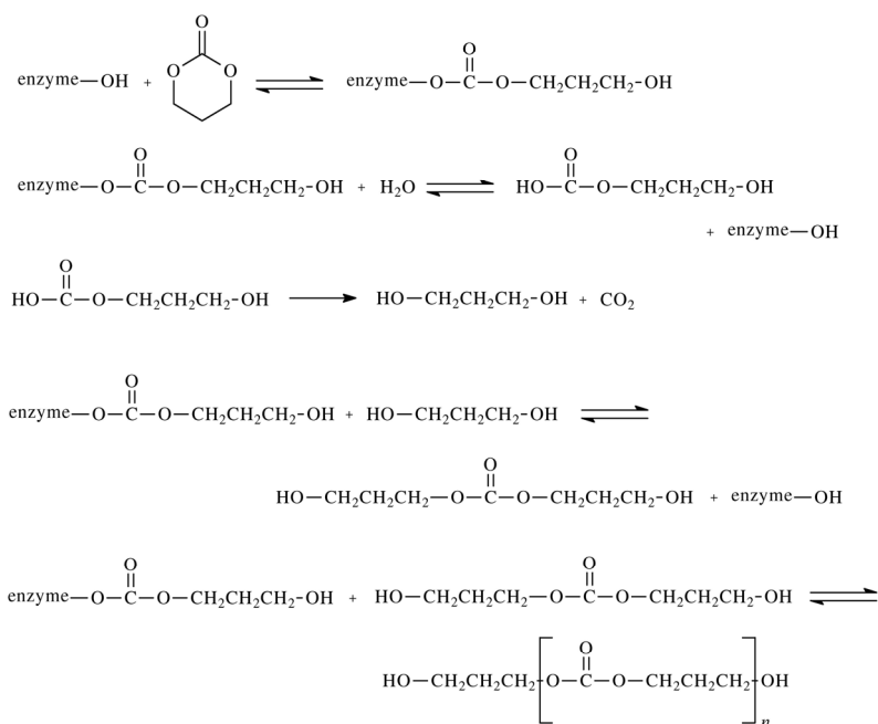
Scheme 2. The mechanism of e-ROP of cyclic carbonates
