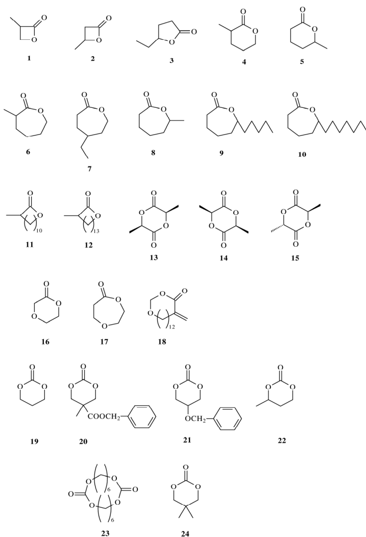
Fig. 5. Representative monomers for e-ROP
