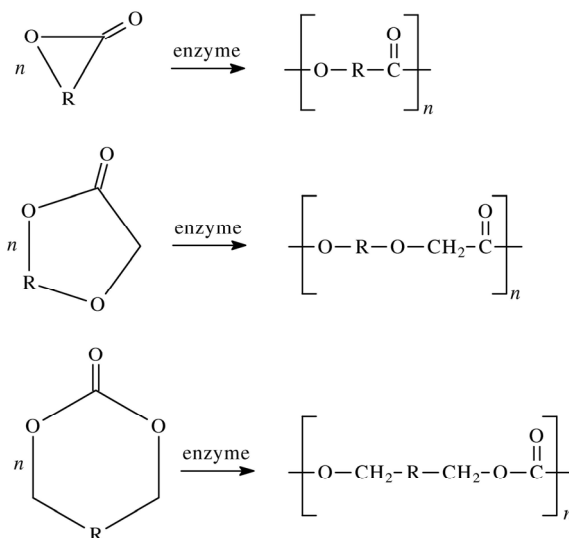
Fig. 4. e-ROP of cyclic esters, ether-esters or carbonates
