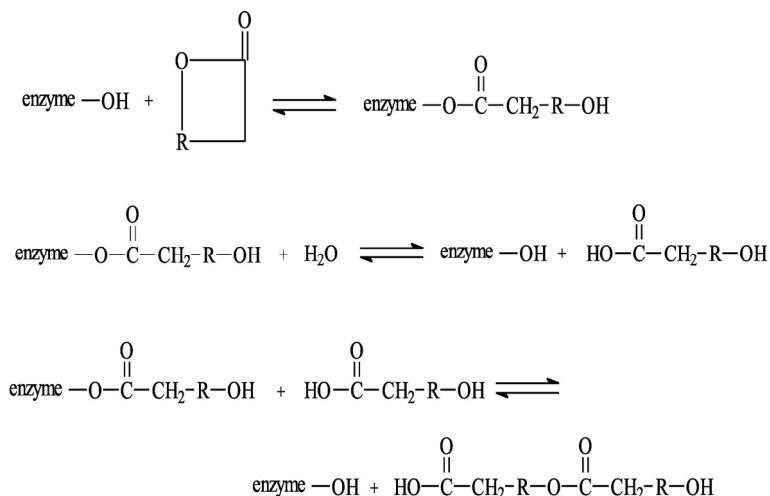
Scheme 1. The mechanism of e-ROP of cyclic esters
