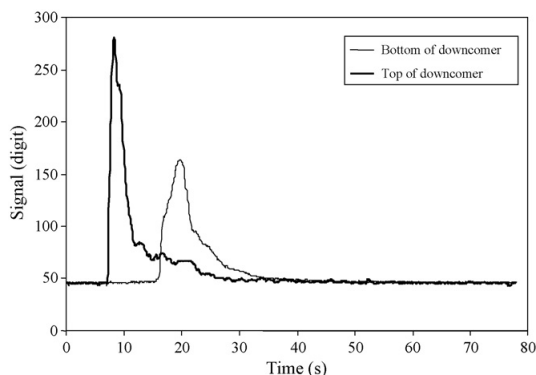
Fig. 13. Example of experimental data from conductivity tracer experiments in the downcomer section when current density j=21.4 mA/cm 2 .
